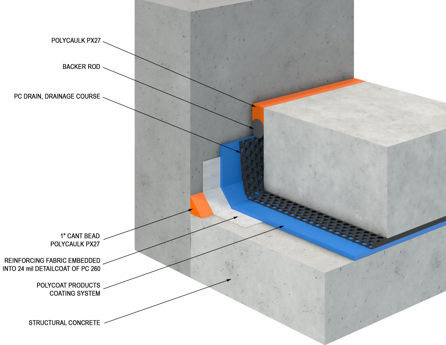
14- BETWEEN SLAB MEMBRANE
