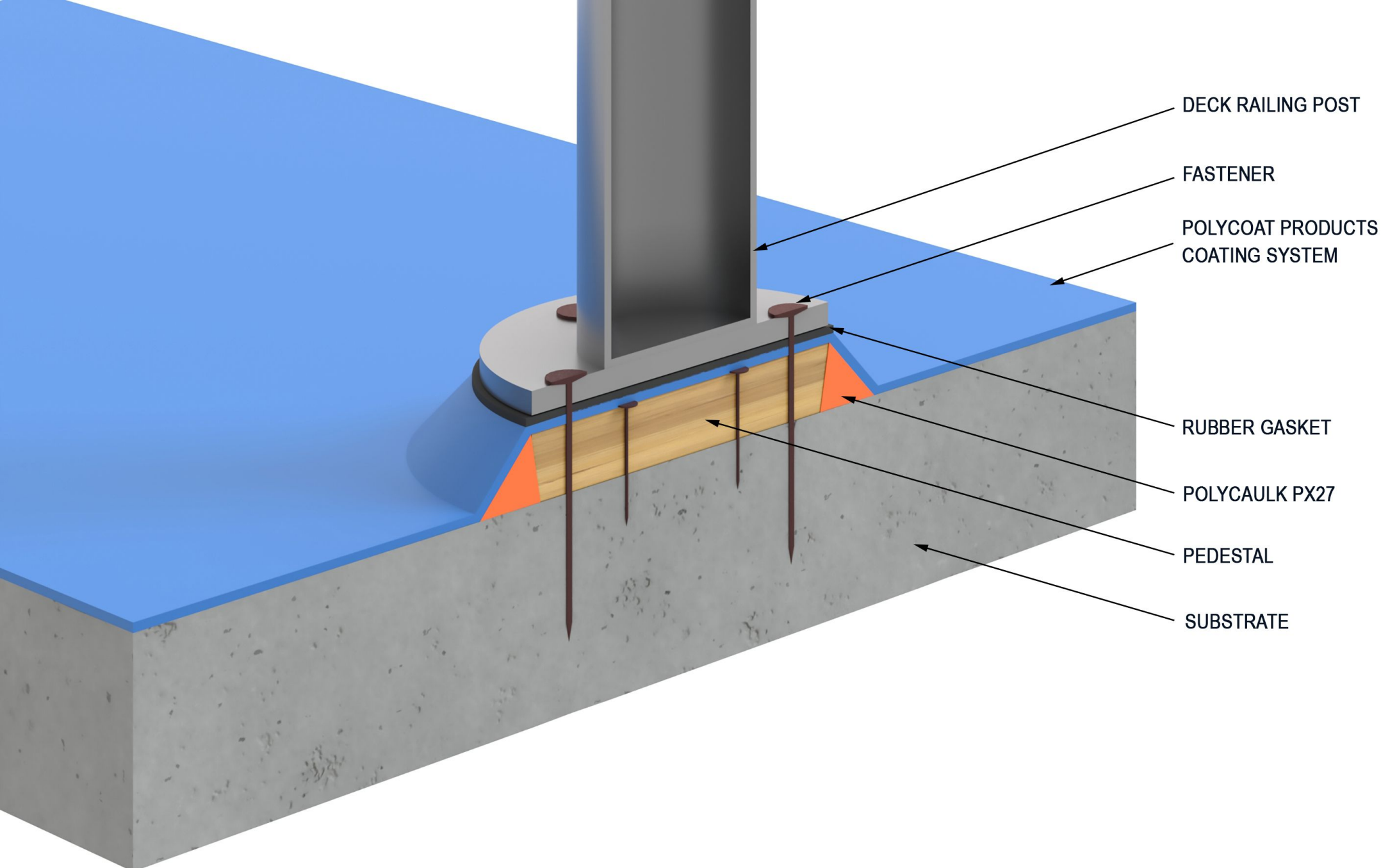
31- DECK RAILING DETAIL
