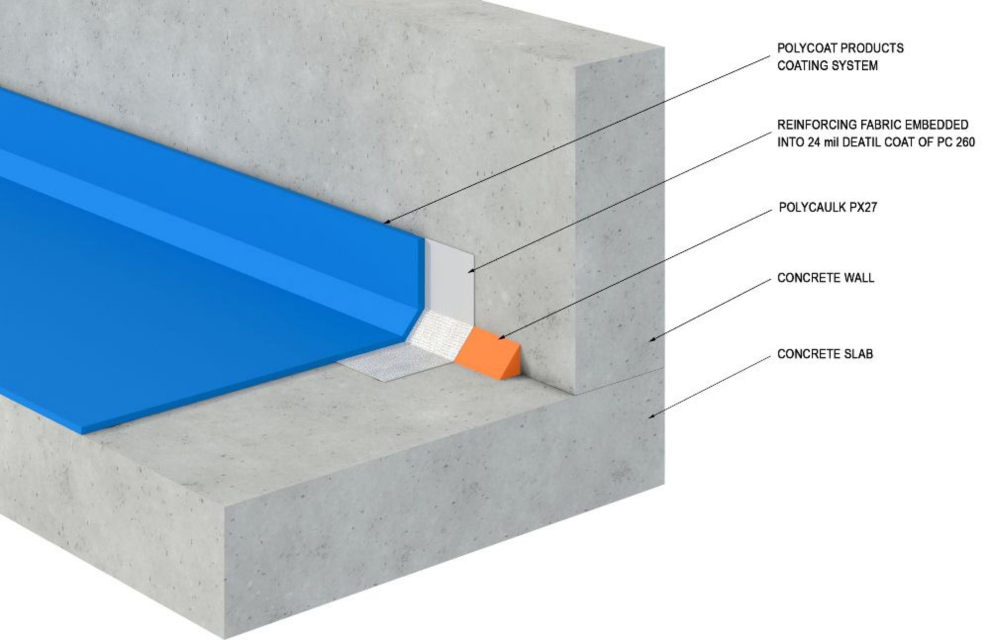
12- WALL BEARING ON SLAB
